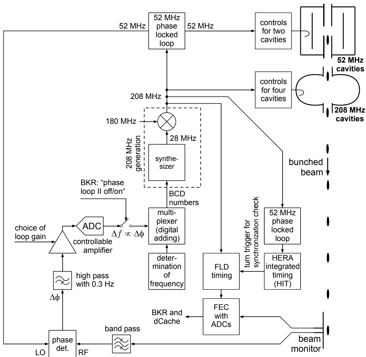
Figure 4.2: The Phase Loop II consists of a narrow band phase detection, whose output is transferred into a change of the frequency values at the RF synthesizer input. The generated 208 MHz RF frequency supplies the cavities controls with RF input signals, partly over a RF phase locked loop. Finally, the loop is closed over the beam. The timing systems use the 208 MHz RF frequency to generate their clock and trigger signals.
