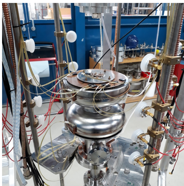
Figure 3: Cavity 16G4 equipped with temperature sensors.
