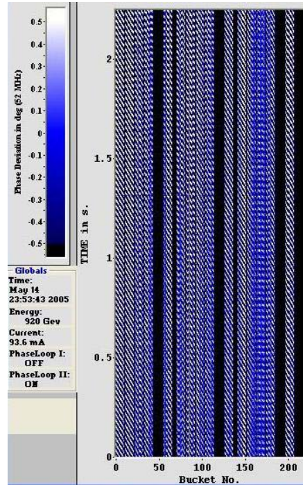
Figure 4: Signature of the mode 164: The pattern shows 512 samples of the bunch phases of all 220 bunch positions.
