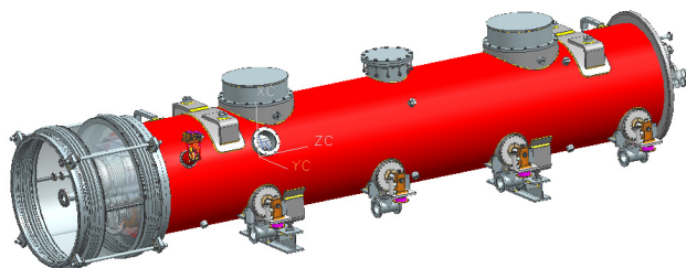
Figure 3: The third harmonic eight cavity module for the EU XFEL.
