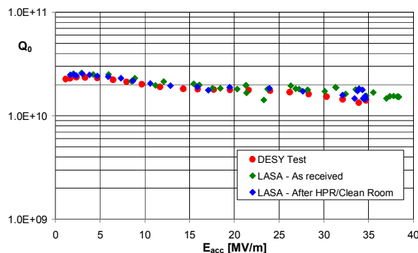
Figure 4: Test history for the qualification of the LASA vertical test area. The 1-cell 1.3 GHz cavity was tested first at DESY and two times at LASA afterwards, as received and after clean room operations and HPR.
