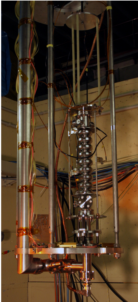
Figure 5: The 3.9 GHz cavity prepared for the test on the variable coupling insert.
