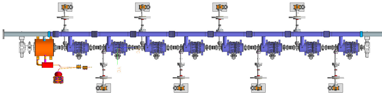
Figure 2: Cavity String layout with alternating coupler configurations and magnet package at the upstream end (beam direction is from left to right). The flange-to-flange cavity string length is 5504 mm.
