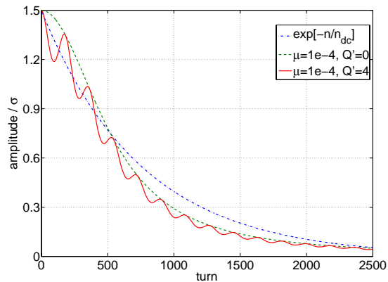
Figure 3: The centre of gravity motion (envelope) of a filamenting bunch without active damping shows different decaying characteristics. A first approximation describes an exponential decaying amplitude (blue, dash-dotted) with parameter \tau_{dc} = 750 turns. The green curve (dashed) accounts for a detuning proportional to r^2 , e.g. octupolar fields, with \mu = 10^{-4} . In case of a non-zero value for the chromaticity and non-vanishing momentum spread the decay is modulated by recoherence (red, solid). Analytical expressions were used [6].
