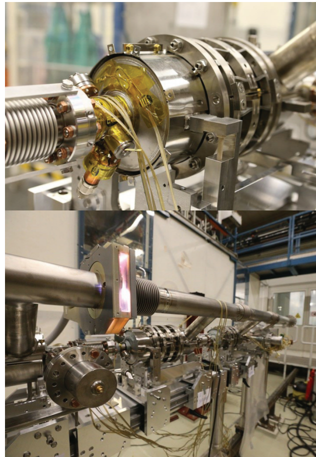
Figure 2: Top: Assembly of the magnetic shielding, blade tuner mechanism and T sensors on the cavity. Bottom: welding operation on the 2 phase line.
