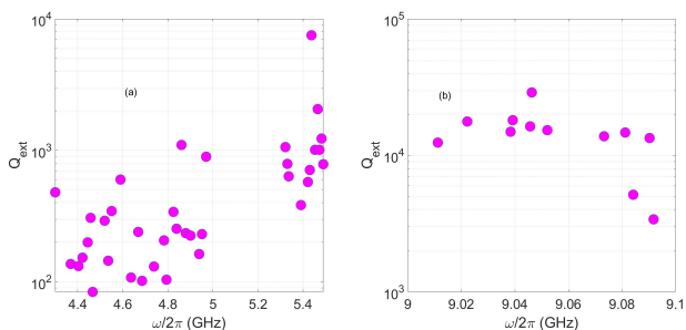
Figure 6: Summary of mode frequencies and external quality factors Q_{ext} for cavity 3HZ010 in superconducting state. (a) First and second dipole band (b) fifth dipole band.
