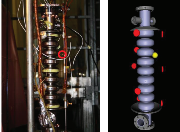
Figure 4. Position of OSTs around the cavity (left photograph of the cavity in the cryostat insert) and reconstruction of the quench origin position (model on the right). The source is highlighted by the red circle on the left and represented by the yellow sphere on the reconstruction picture, where OSTs are shown in red.
