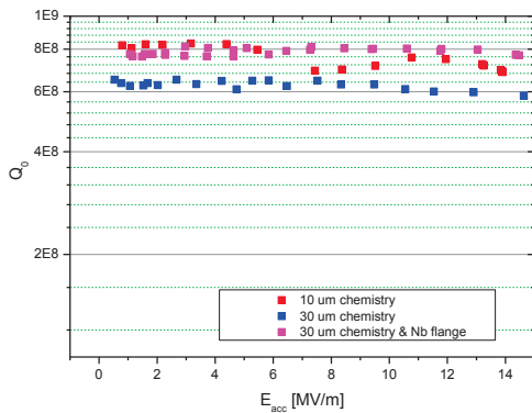
Figure 1. Q_0 versus E_{acc} for cavity 3HZ02 in three tests following different treatments: 10 \mu\text{m} BCP, 10+20 \mu\text{m} BCP and after installation of a Nb-sputtered flange. In all cases, the maximum field at 15 MV/m was limited by a hard cavity quench, in absence of X-Ray and field emission activity. Test temperature is 2.0 K (31 mbar).
