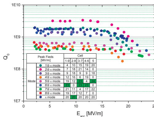
Figure 3. Q_0 vs E_{acc} for all fundamental pass-band modes of cavity 3HZ03. The mode analysis shows that cells #2 and #8 are limiting the cavity performance in the \pi mode, while the other individual cells reach 23 MV/m and above (values highlighted in green).
