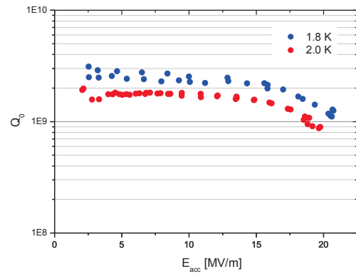
Figure 2. Q_0 versus E_{acc} for cavity 3HZ03 at 2.0 K and 1.8 K. The cavity is limited by quench without X-ray or field emission.
