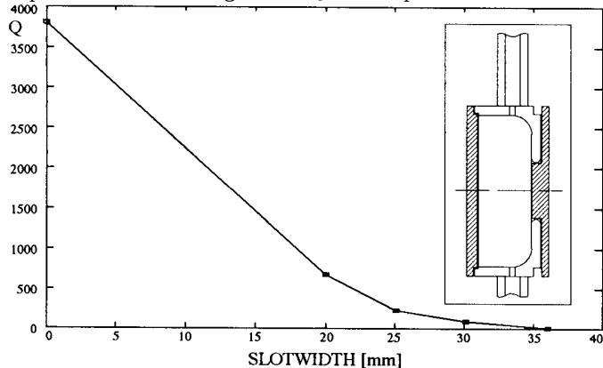
Figure 2: Single damper cell Q-value versus slotwidth.
