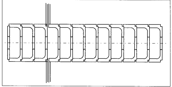
Figure 3: Damped 12-cell structure.
