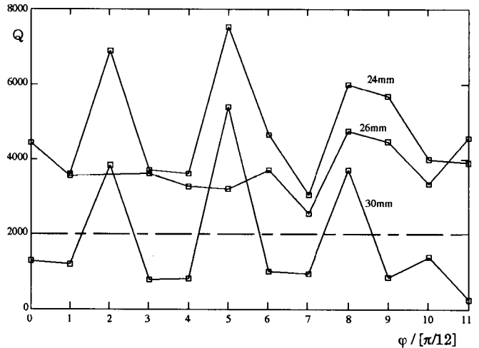
Figure 4: Measured Q-values of the first dipole passband.
