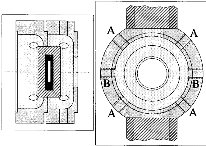
Figure 1: Damper cell with two waveguides.
