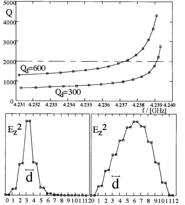
Figure 7: Calculated Q-value of the 11/12\pi -dipole-mode and related field distributions.
