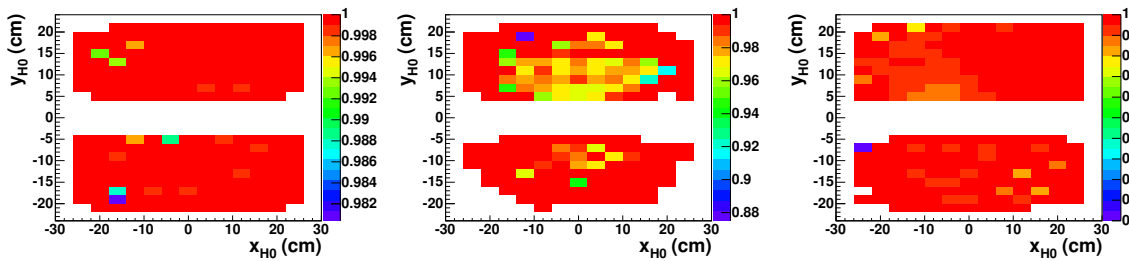
Figure 5.35: H0 efficiency (in color) in 2002 (left), 2003 (center) and 2004 (right).
