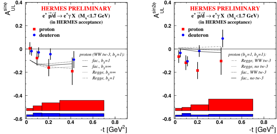
Figure 3.5: Longitudinal target-spin asymmetry A_{UL} on the proton and deuteron measured at HERMES [Kop05]. The A_{UL}^{\sin \phi} amplitude is shown as a function of -t , after background correction. Error bars and bands represent the statistical and systematic uncertainties, respectively. The curves shown are calculations based on GPD models [Goe01] for the proton, using either a factorized or a Regge inspired t -dependence with or without twist-three effects in the Wandzura-Wilczek (WW) approximation [Goe01].
