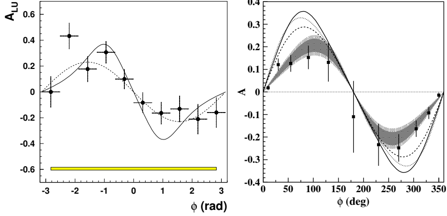
Figure 3.4: Beam-spin asymmetry A_{LU} on the proton measured at HERMES (left panel) [Air01] and CLAS (right panel) [Ste01]. Left: the dashed curve represents a \sin \phi dependence with an amplitude of 0.23, while the solid curve represents the result of a model calculation at twist-three level from Ref. [Kiv01]. The error band below shows the systematic uncertainty. Right: the shaded regions represent the experimental results, while the curves represent model calculations from Refs. [Van99, Goe01]. The dashed (dotted) curve is a calculation with \xi -independent ( \xi -dependent) GPDs at leading-twist. The solid curve includes twist-three effects.
