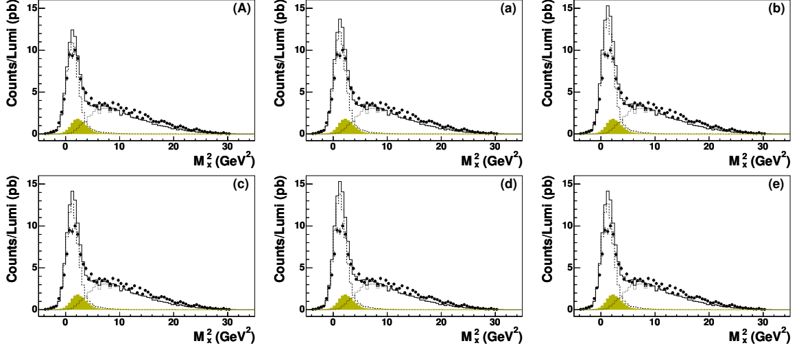
Figure 5.7: Same as Fig. 5.5 but the reconstructed photon energies in the MC simulation are decreased by 1%.
