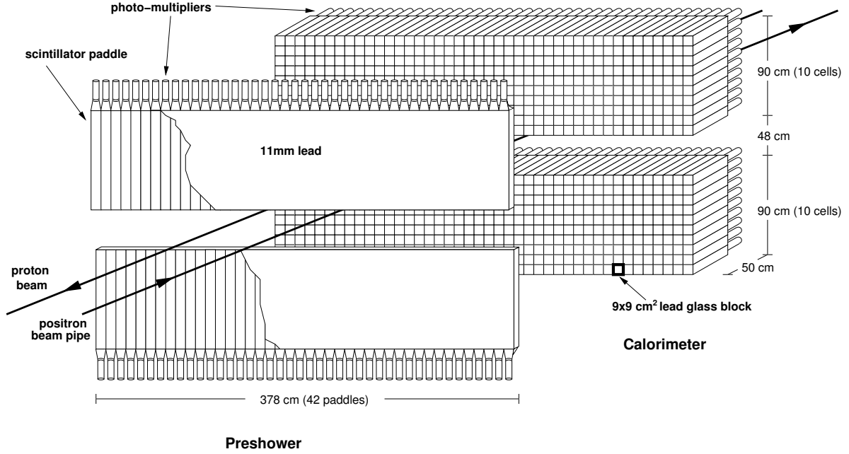
Figure 4.6: Schematic view of the calorimeter and the pre-shower detector.
